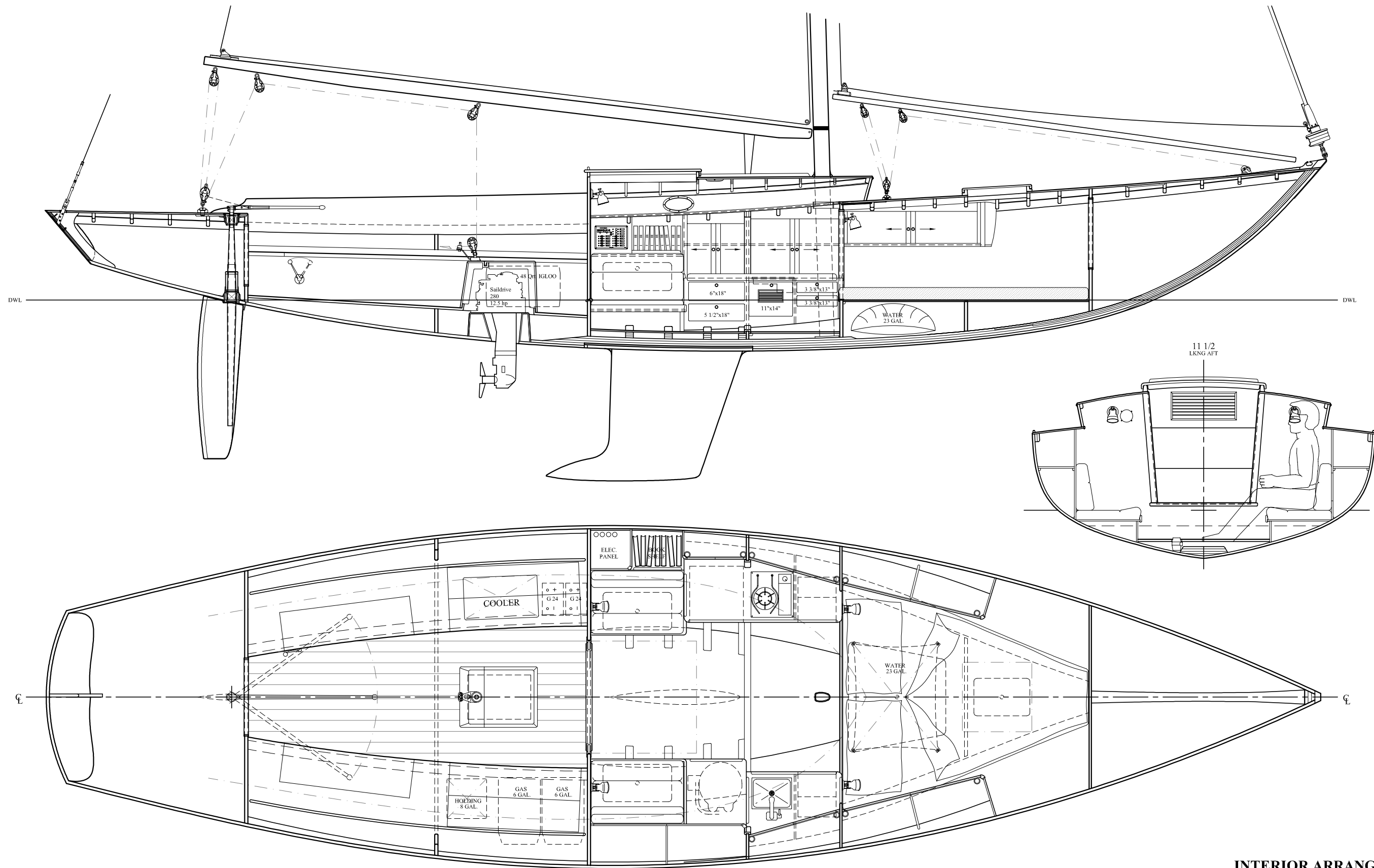
INTERIOR ARRANGEMENT 34' Daysailer SKYLARK
