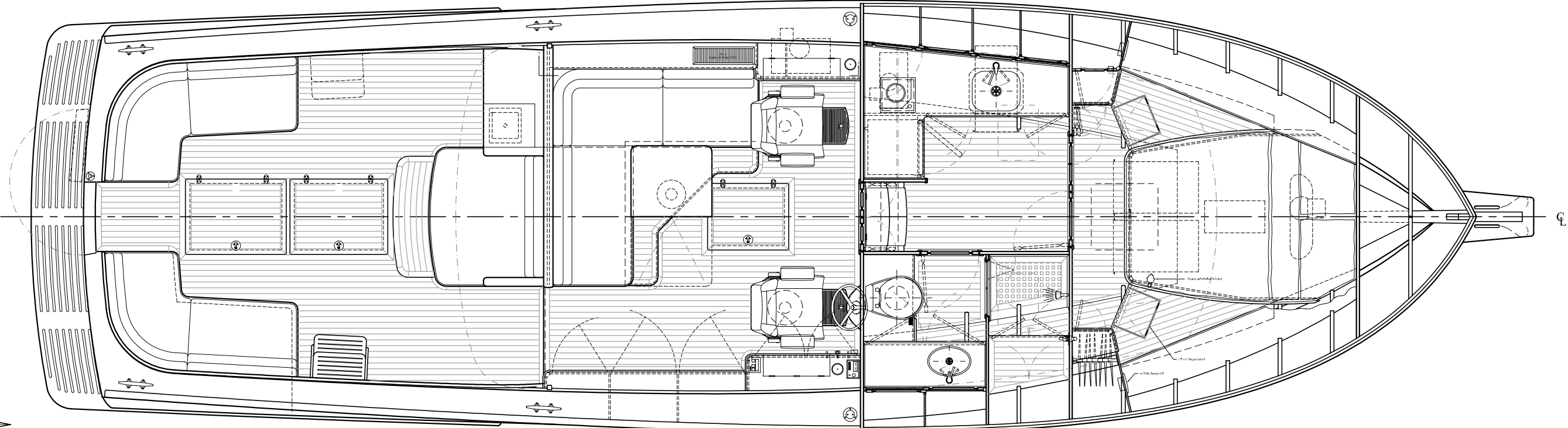
40' MONOMOY EXPRESS SOLIPSYS Interior Arrangement
