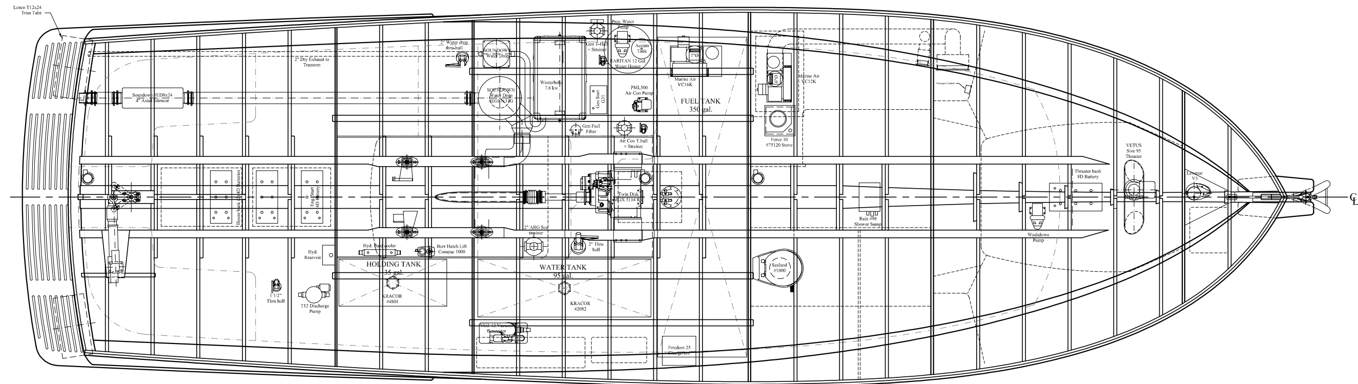
40' MONOMOY EXPRESS SOLIPSYS Mechanical Arrangement
